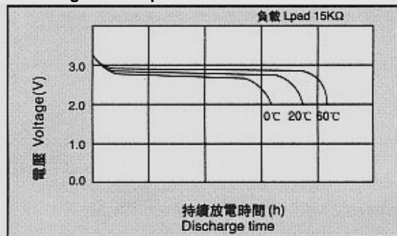
Discharge on Temperature
