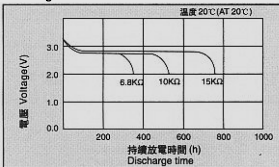
Discharge on Load
